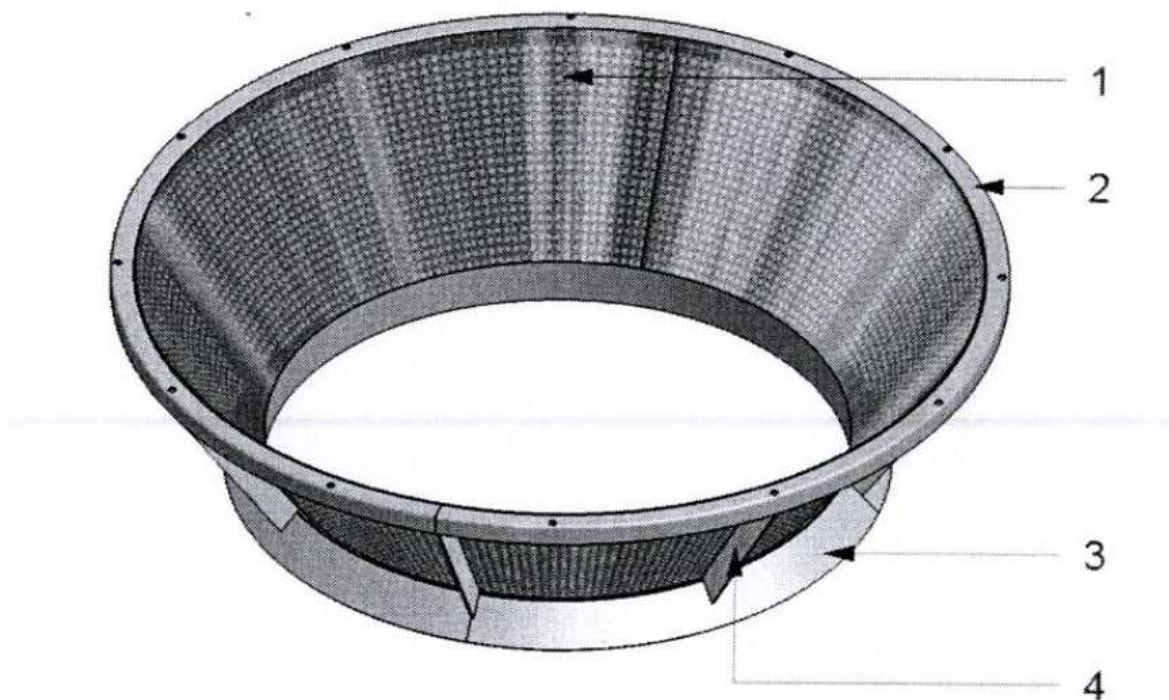
Fig. 4-5 Strainer basket
